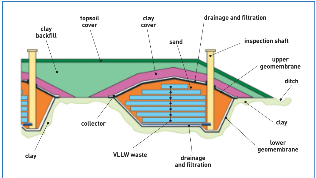
Figure 3. Cross-section of a disposal pit for VLLW waste.
