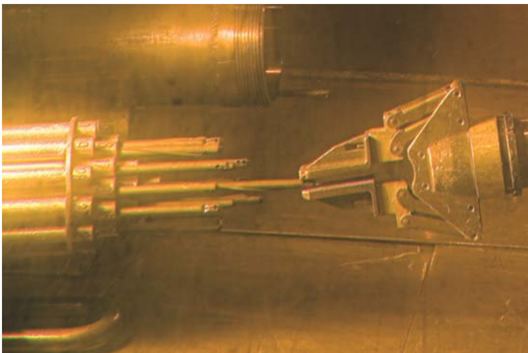
Nondestructive investigation of an ECRIX-H experimental pin, inside a Phénix shielded cell, after irradiation, and cooling of the experiment.
