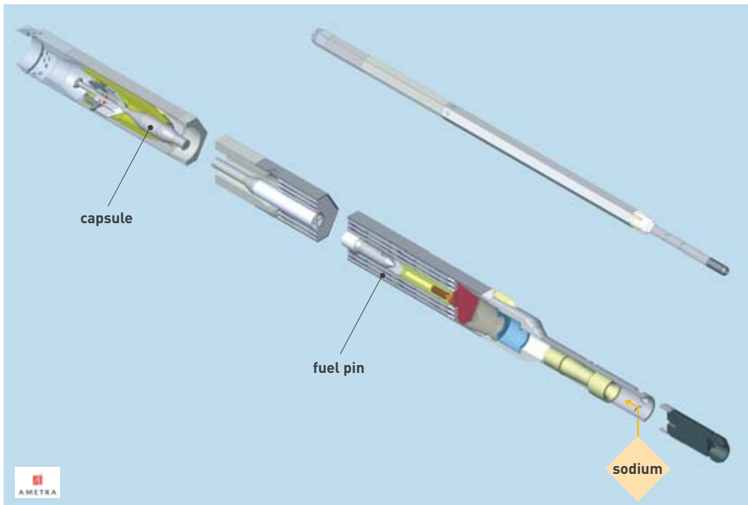
Figure 1. Irradiation device. The pins, or internal components holding the fuels, or materials to be tested are inserted into, and positioned in the experimental capsule. The capsule is then locked into its holder.
