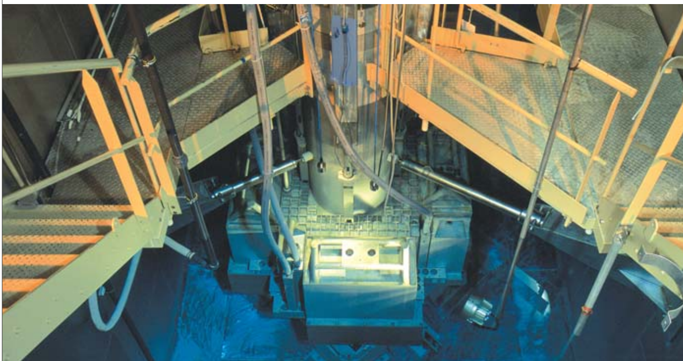
A view of the MELODIE core, in the pool of the MINERVE reactor.
