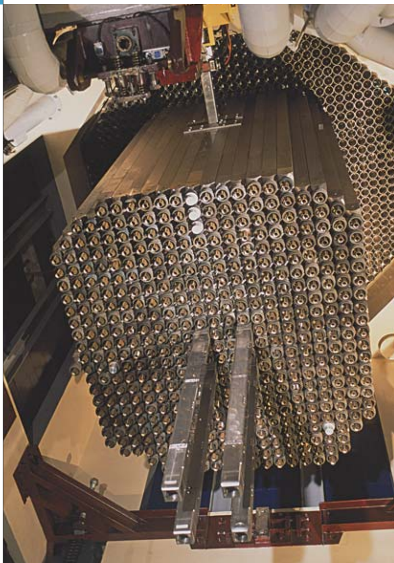
The MASURCA reactor core, seen from below.
